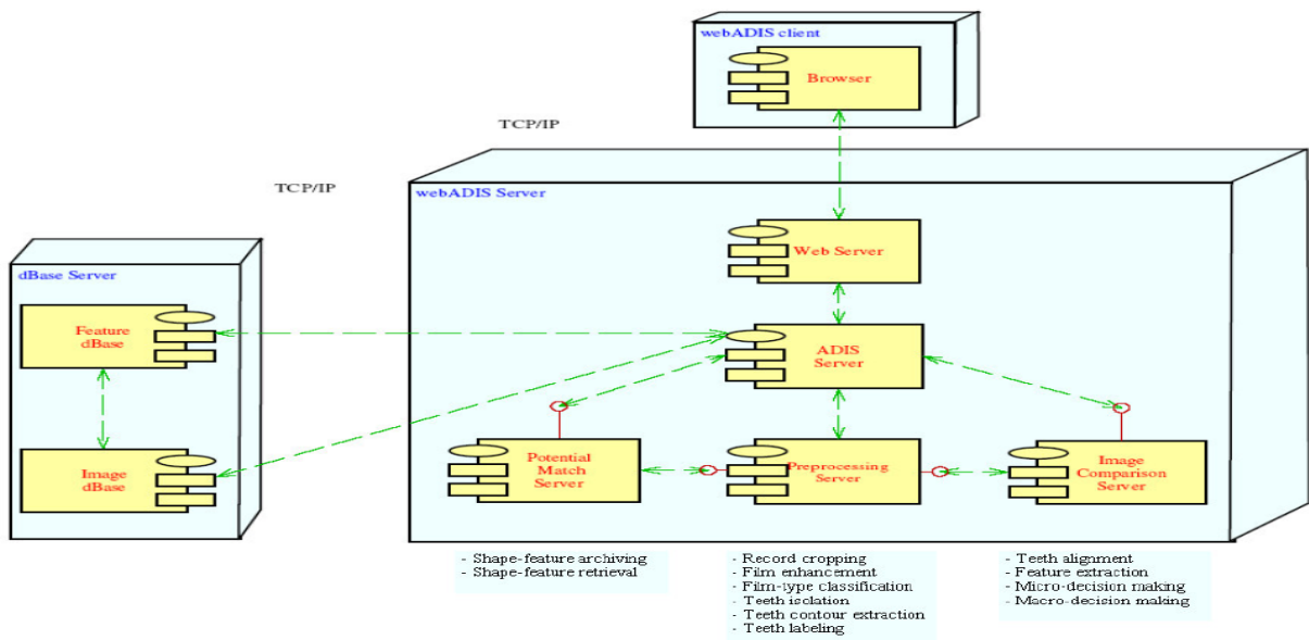
Figure 1: Architecture of webADIS; the web accessible ADIS environment.
