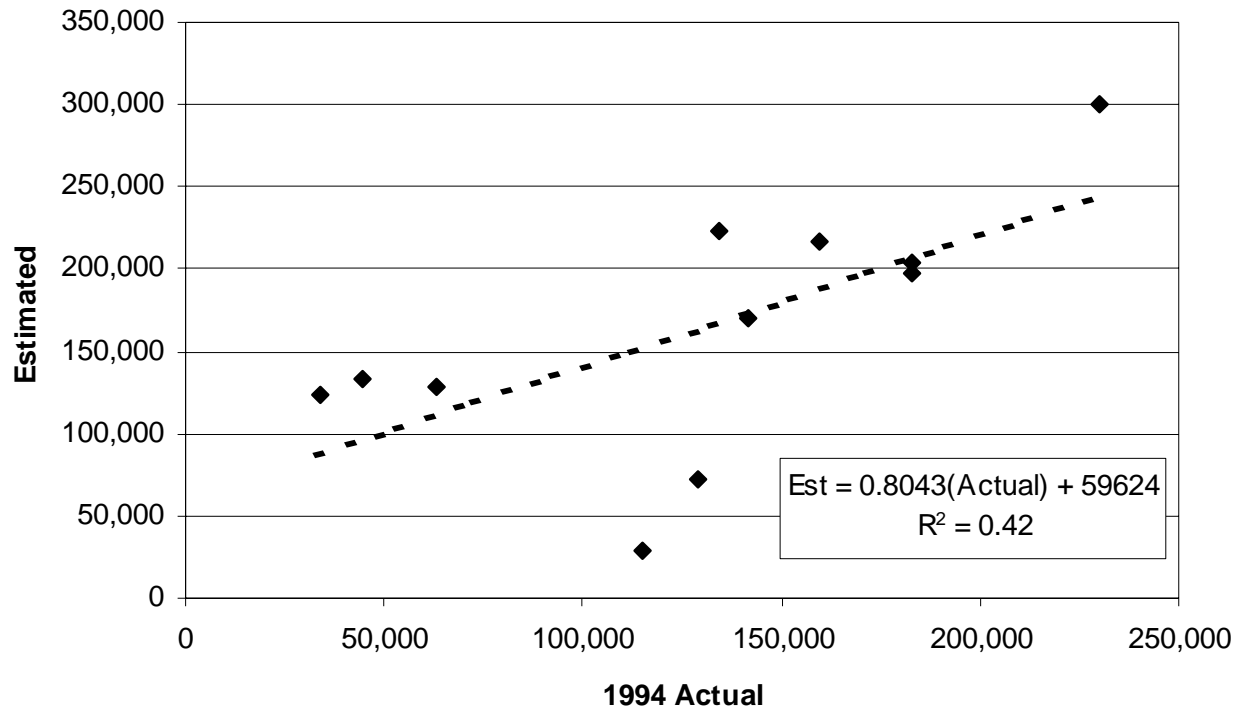
Estimated and Actual Screenline HDT, 24 hour, in PCEs
